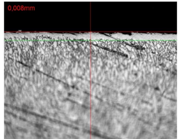
Fig. 4: light optical micrograph of an Expanite-hardened Stellite 1040 showing a hardened zone of ca. 8 \mu m. Surface hardness measurements resulted in ca. 900HV0.025
