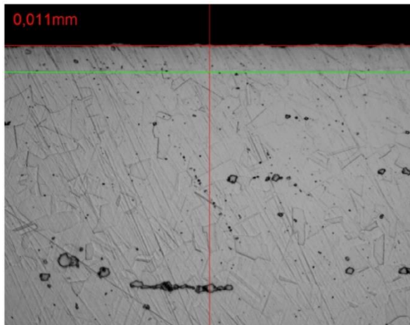
Fig. 3: light optical micrograph of an Expanite-hardened Inconel 718 evidencing a homogenous case-depth in the range of ca. 10 \mu m. Surface hardness measurements reveal ca. 1,000 HV0.025
